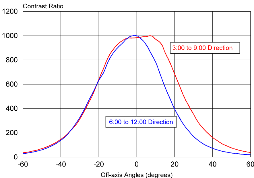
LM216C-150X1-AR LCD Contrast Ratio Angular Distribution
