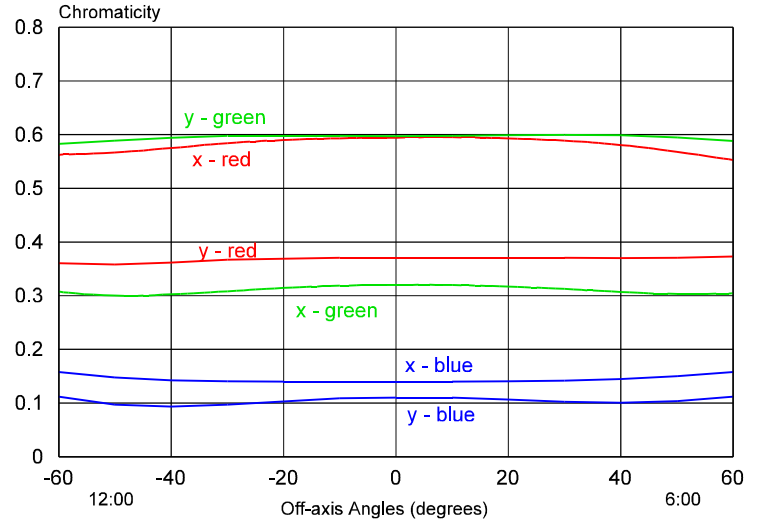
LM216C-150X1-AR Color Shift along the 6:00 - 12:00 Directions (Positive Angles are along the 6:00 Direction)
