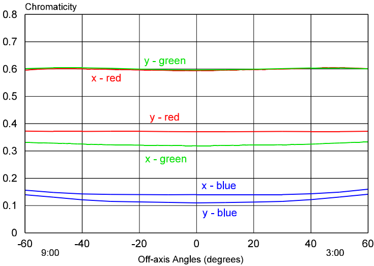
LM216C-150X1-AR Color Shift along the 3:00 - 9:00 Directions (Positive Angles are along the 3:00 Direction)
