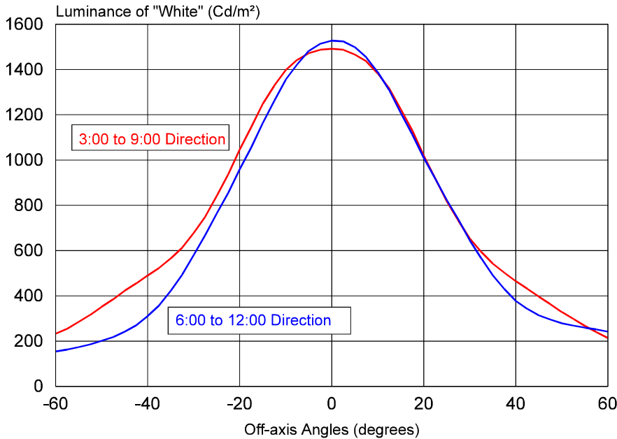
LM216C-150X1-AR Screen Luminance Angular Distribution
